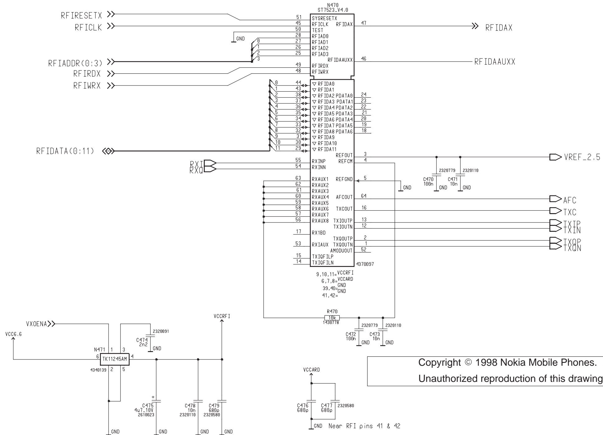
Regulator for RFI2 analog supply
